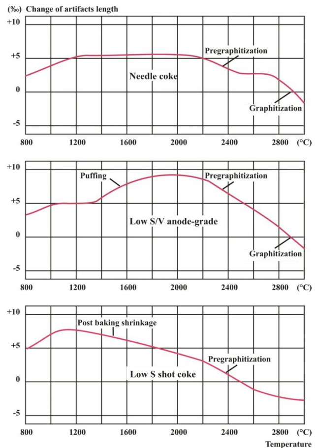
Figure 3. Graphitization dilatometric curves of pet cokes
