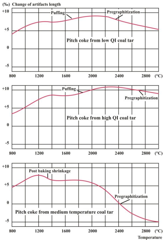
Figure 4. Graphitization dilatometric curves of pitch cokes
